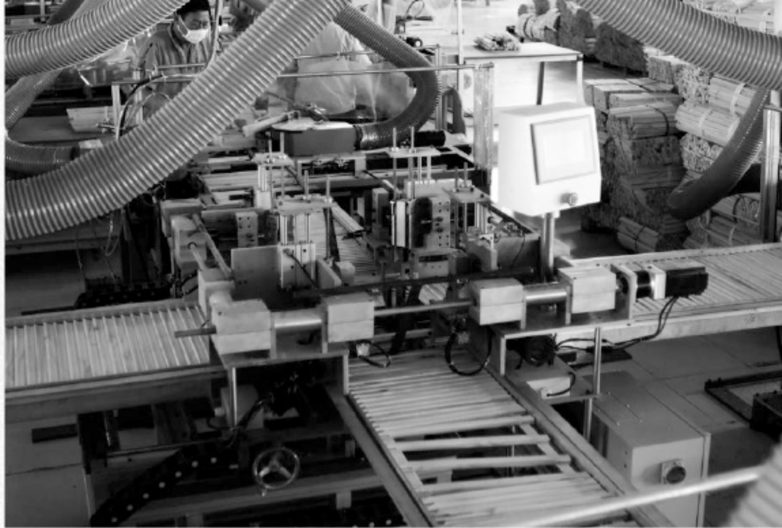
Automatic tenoning line
